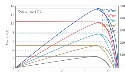
I-V curves/P-V curves at different irradiance (420W)
