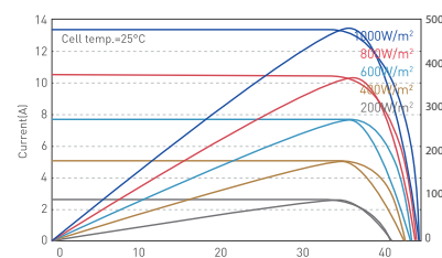
I-V curves/P-V curves at different irradiance (465W)
