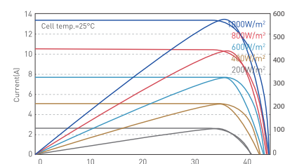
I-V curves/P-V curves at different irradiance (510W)
