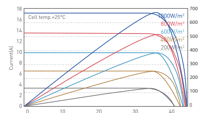
I-V curves/P-V curves at different irradiance (615W)
