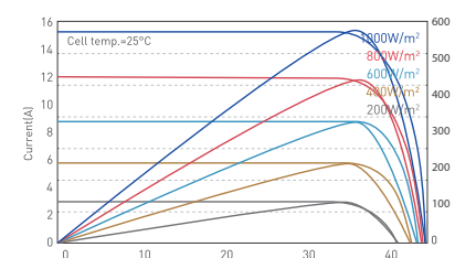
I-V curves/P-V curves at different irradiance (515W)
