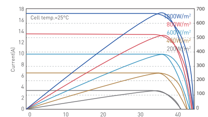
I-V curves/P-V curves at different irradiance (670W)
